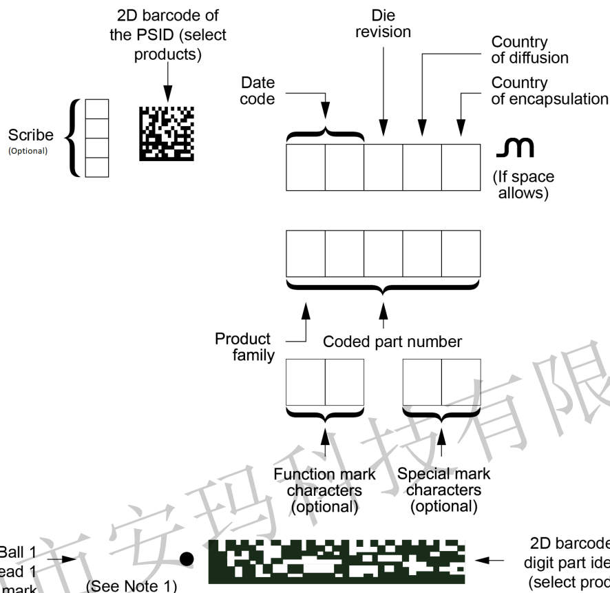
Figure 2: SOP2/W-PDFN/BGA/LGA Abbreviated Component Mark
